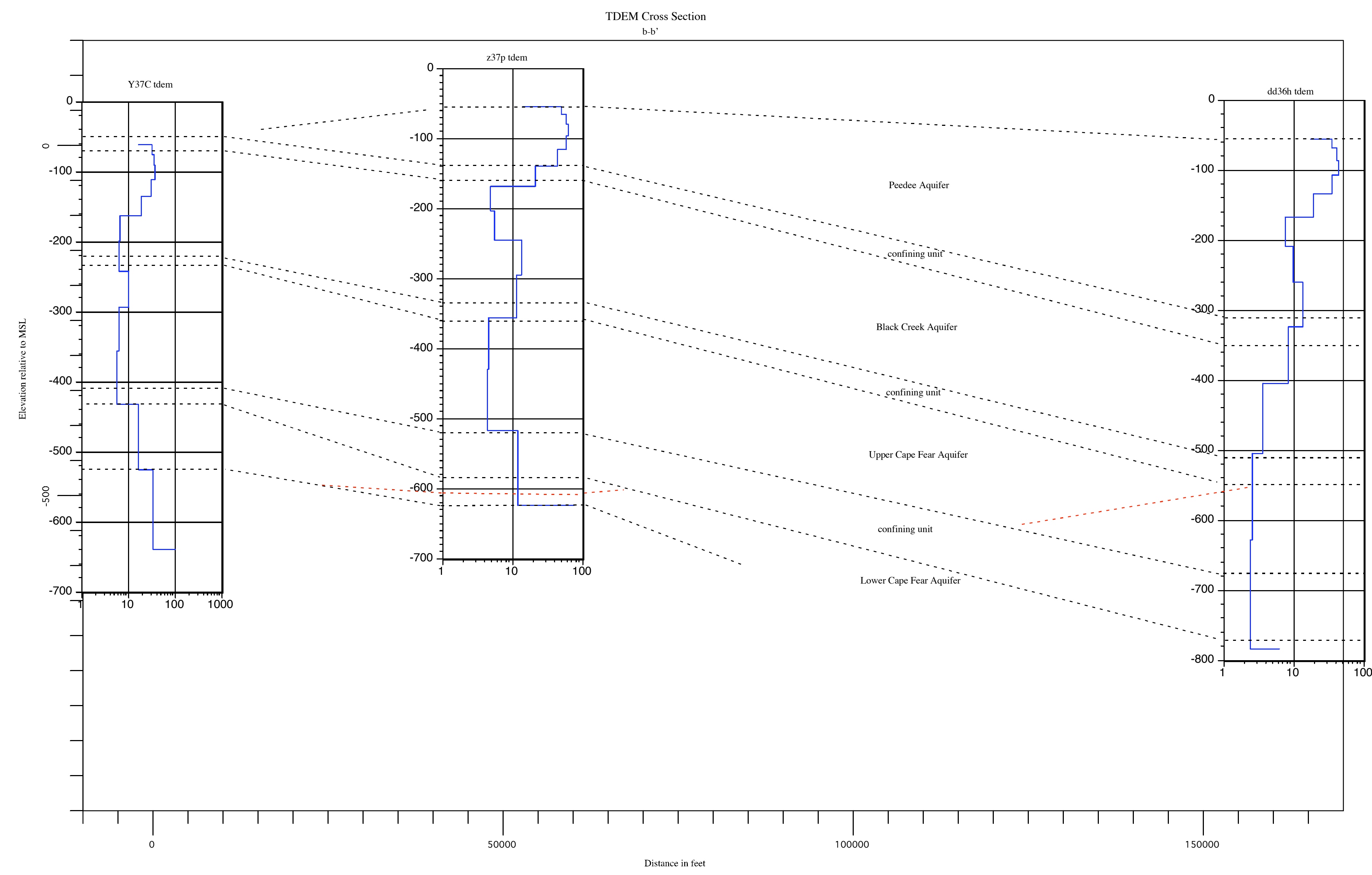
Plate 25. Time Domain Electromagnetic Resistivity Profile b-b' through Bladen, Brunswick and Columbus Counties, NC
